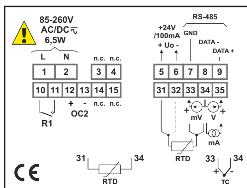
version with 1 x REL and 1 x OC (SSR)
