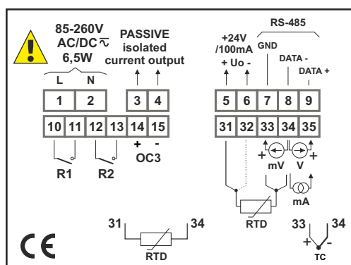
version with 2 x REL, 1 x OC (SSR) and 1 x AO 4-20 mA, passive
