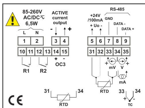
version with 2 x REL, 1 x OC (SSR) and 1 x AO 0/4-20 mA, active
